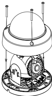
Figure 2-10 Instalați bula
